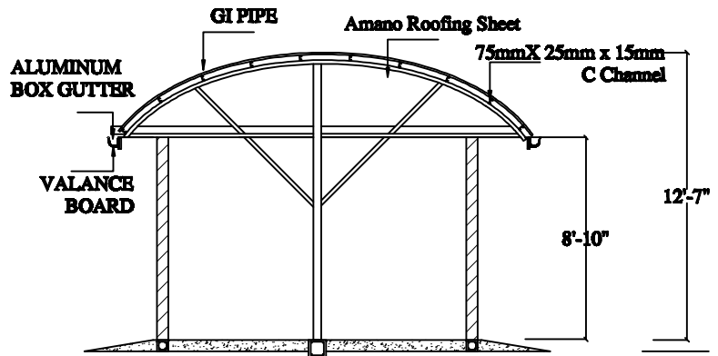
SECTION X-X
